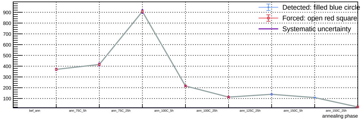
Sensor A1, v = 5 V, T = 23 °C - Spot 87: luminosity vs phase
