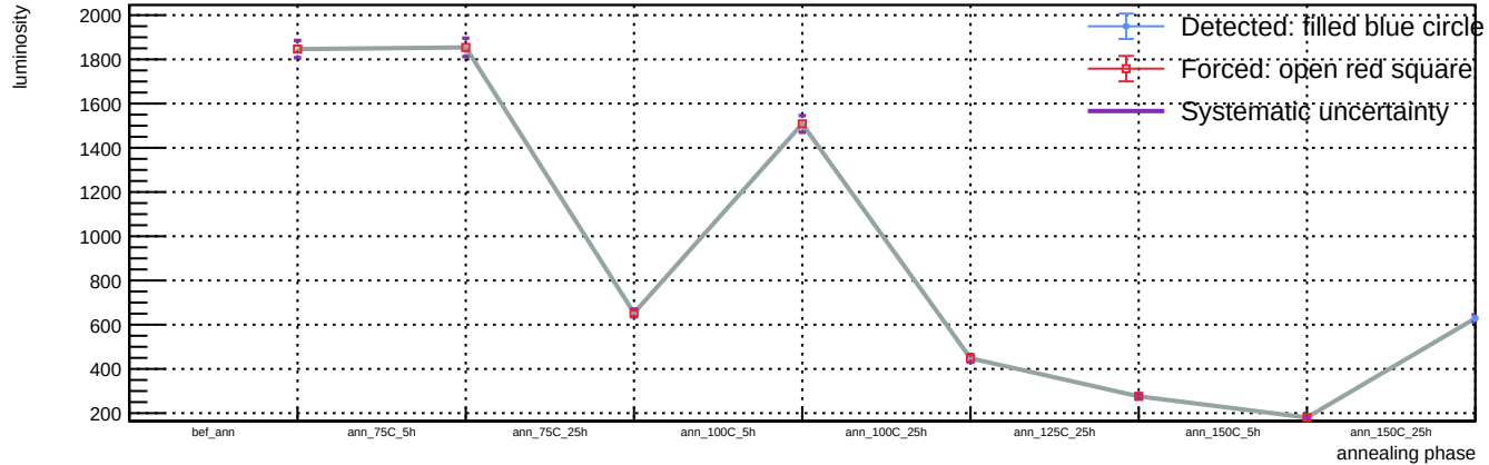
Sensor A1, v = 5 V, T = 23 °C - Spot 88: luminosity vs phase
