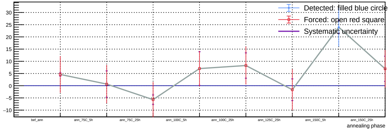
Sensor A1, v = 5 V, T = 23 °C - Spot 89: luminosity vs phase
