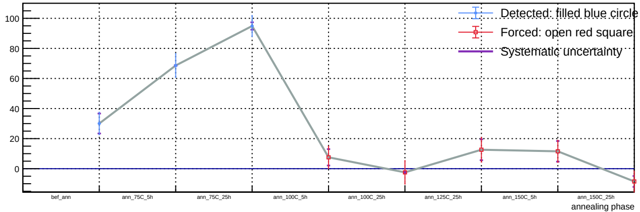
Sensor A1, v = 5 V, T = 23 °C - Spot 9: luminosity vs phase
