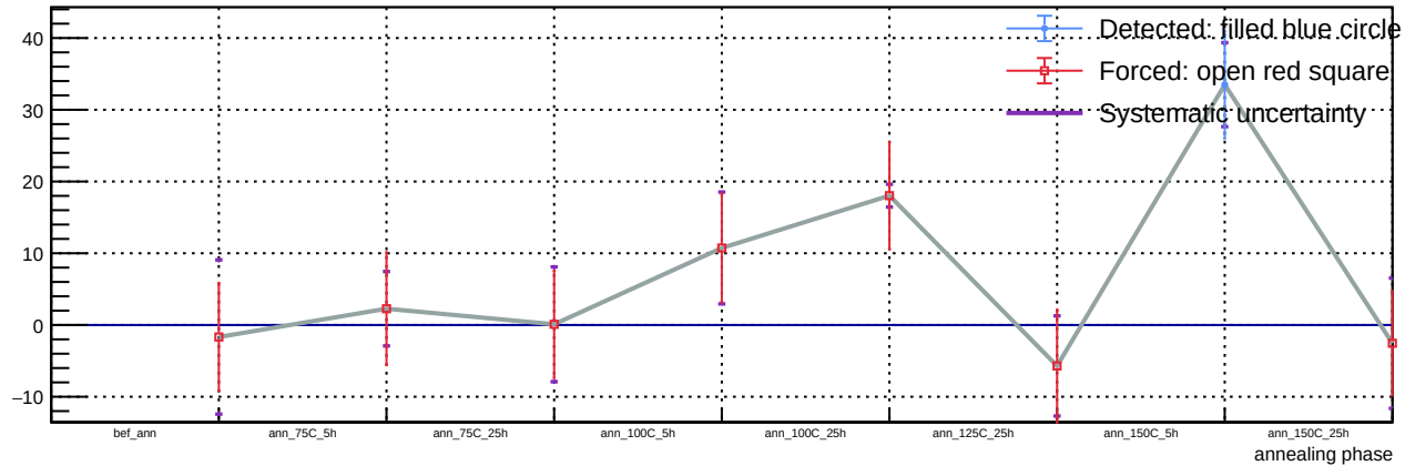
Sensor A1, v = 5 V, T = 23 °C - Spot 90: luminosity vs phase
