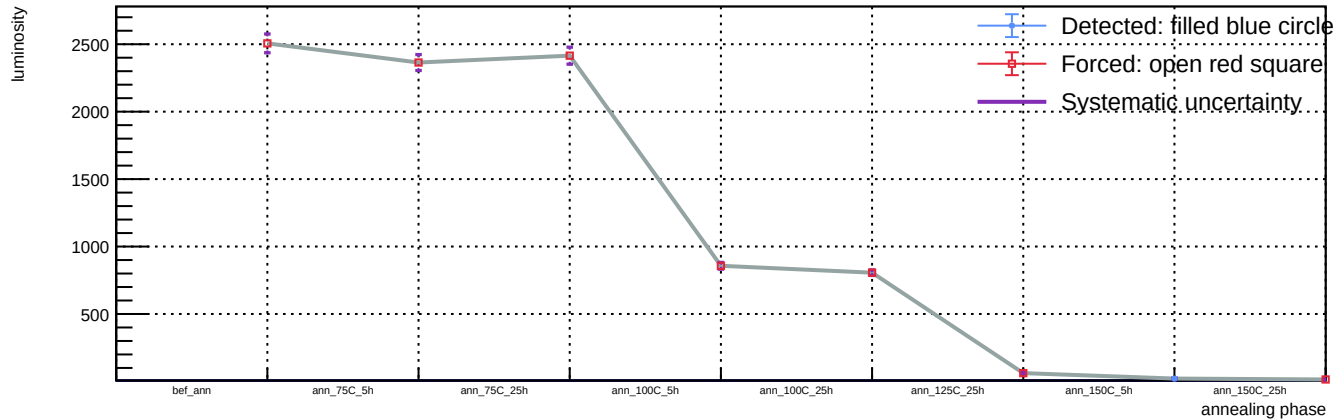
Sensor A1, v = 5 V, T = 23 °C - Spot 91: luminosity vs phase
