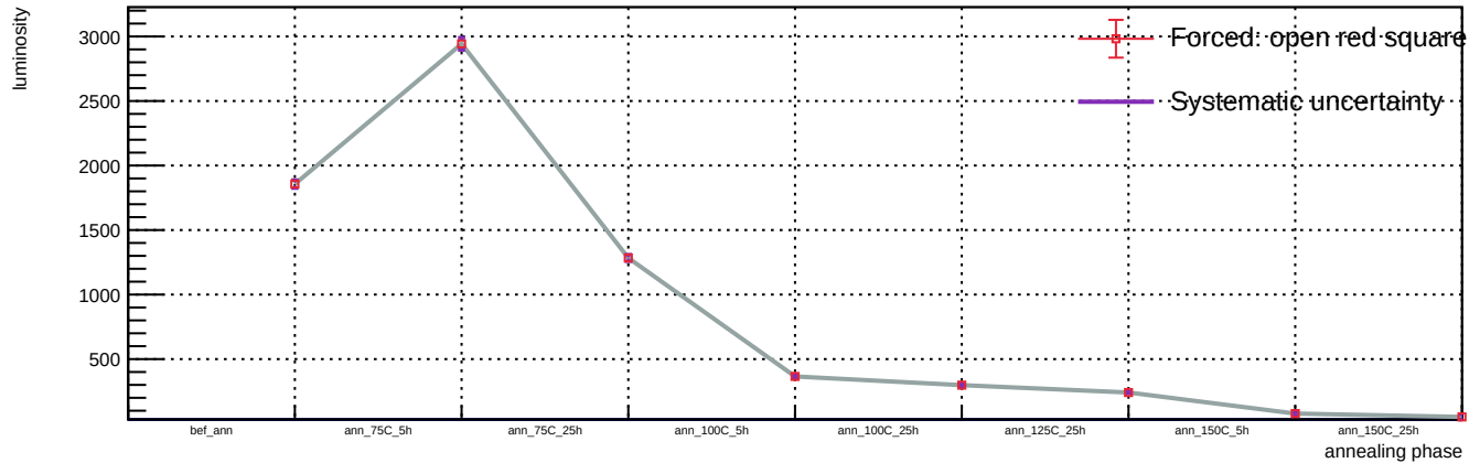
Sensor A1, v = 5 V, T = 23 °C - Spot 92: luminosity vs phase
