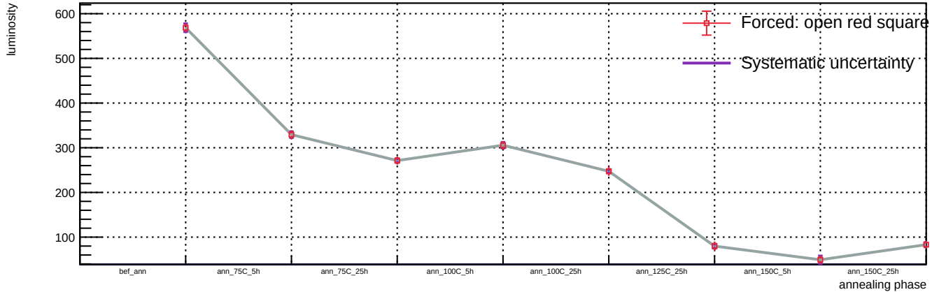
Sensor A1, v = 5 V, T = 23 °C - Spot 93: luminosity vs phase
