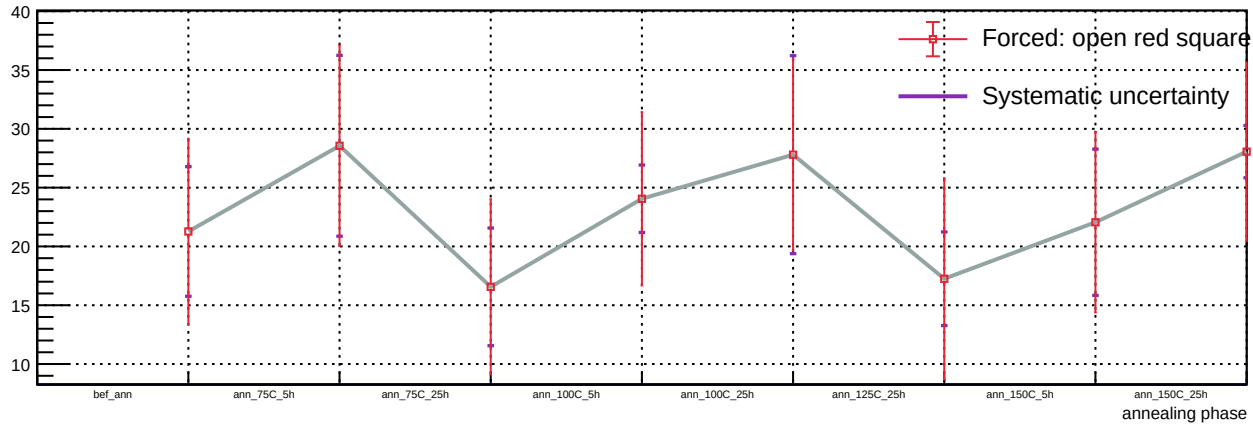
Sensor A1, v = 5 V, T = 23 °C - Spot 94: luminosity vs phase
