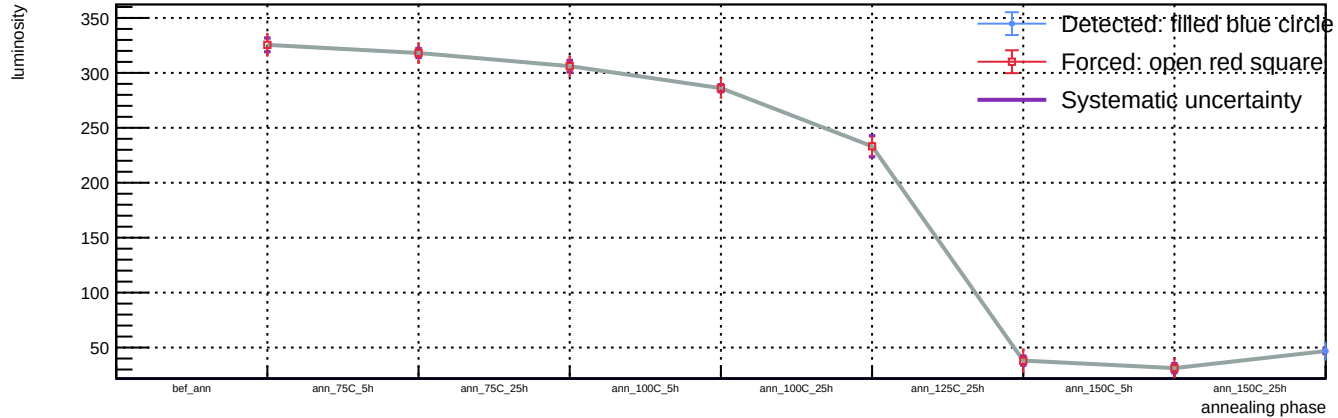
Sensor A1, v = 5 V, T = 23 °C - Spot 95: luminosity vs phase
