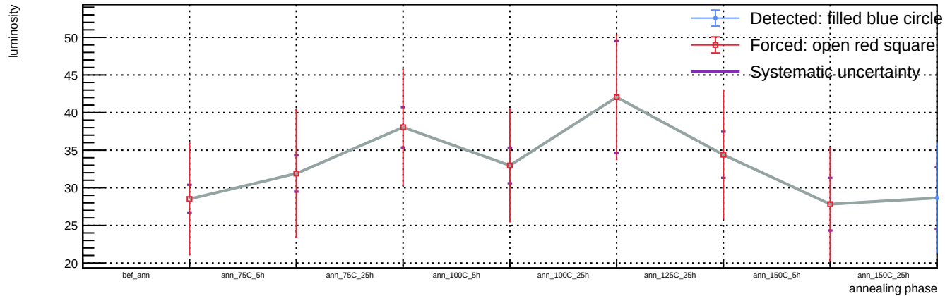
Sensor A1, v = 5 V, T = 23 °C - Spot 96: luminosity vs phase
