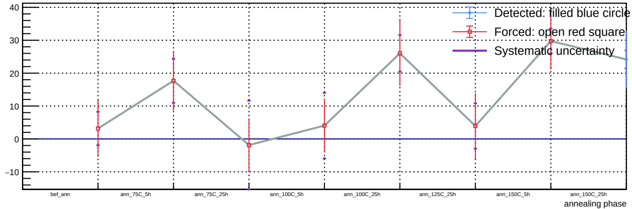
Sensor A1, v = 5 V, T = 23 °C - Spot 97: luminosity vs phase
