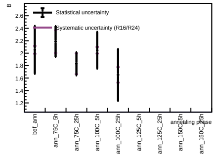
Sensor B1, T = 20 C - Spot 47
