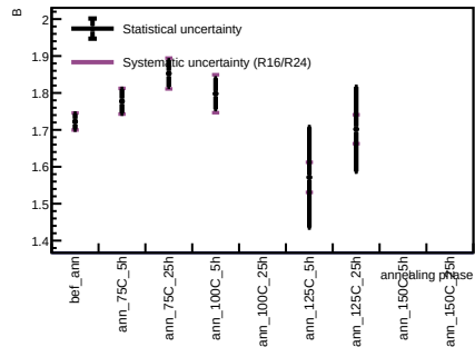
Sensor B1, T = 20 C - Spot 42
