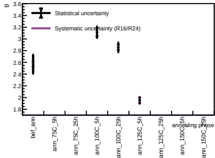
Sensor B1, T = 20 C - Spot 43
