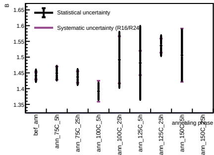
Sensor B1, T = 20 C - Spot 45
