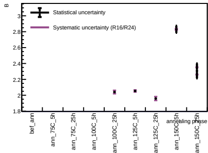
Sensor B1, T = 20 C - Spot 63
