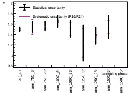
Sensor B1, T = 20 C - Spot 61
