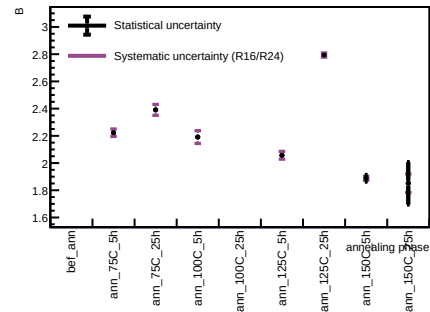
Sensor B1, T = 20 C - Spot 65
