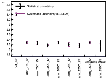
Sensor B1, T = 20 C - Spot 60
