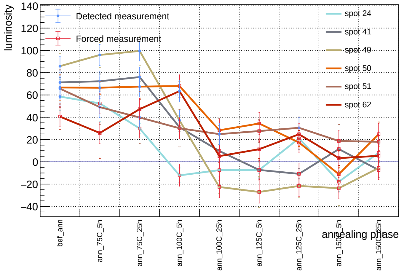
Sensor B1, T = 20 C, v_{\text{over}} = 5 \text{ V} - luminosity vs phase - order 10^1
