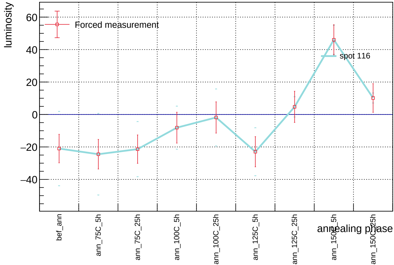
Sensor B1, T = 20\text{ C} , v_{\text{over}} = 5\text{ V} - luminosity vs phase - order 10^1
