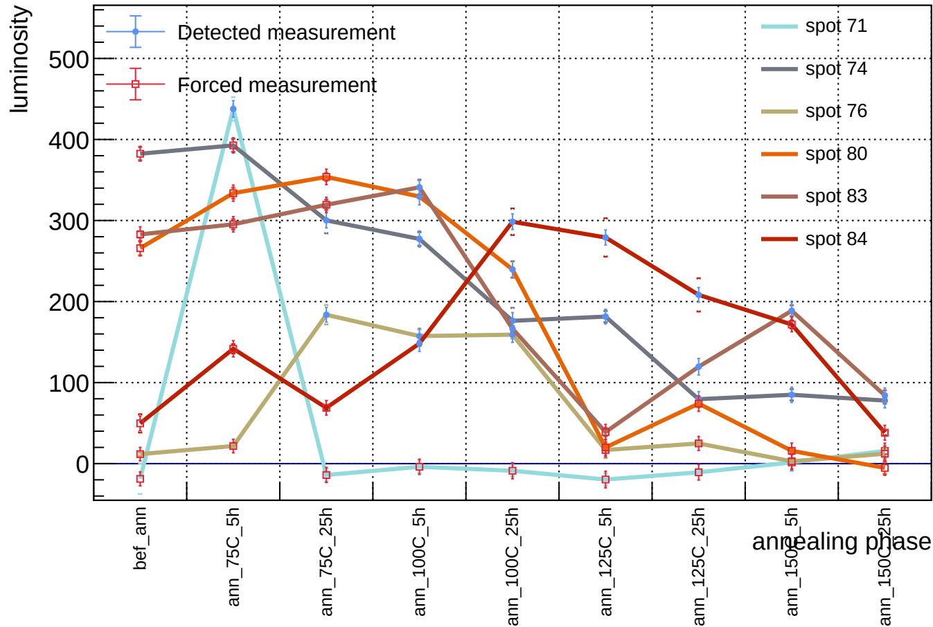
Sensor B1, T = 20\text{ C} , v_{\text{over}} = 5\text{ V} - luminosity vs phase - order 10^2
