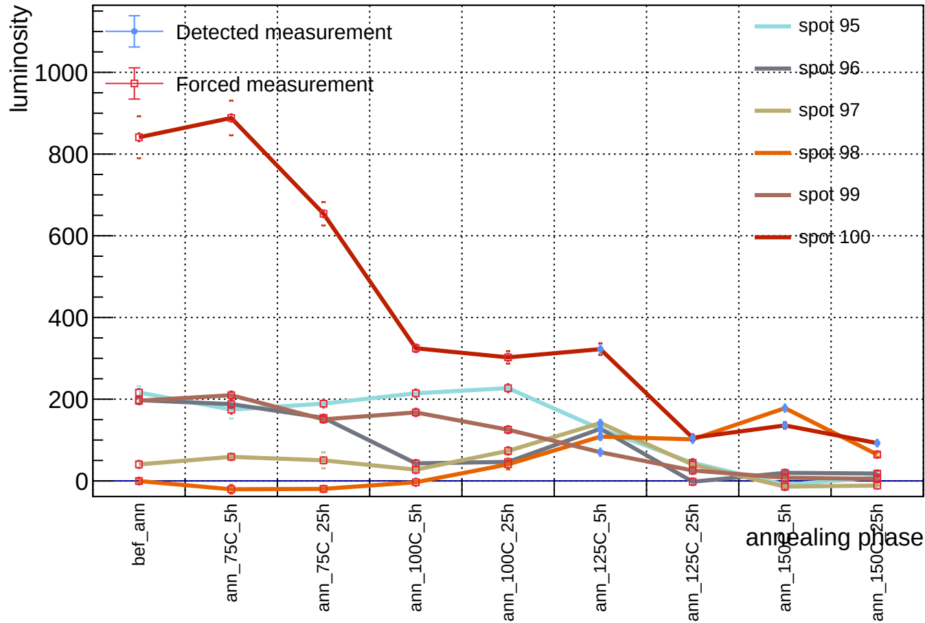
Sensor B1, T = 20 C, v_{\text{over}} = 5 \text{ V} - luminosity vs phase - order 10^2
