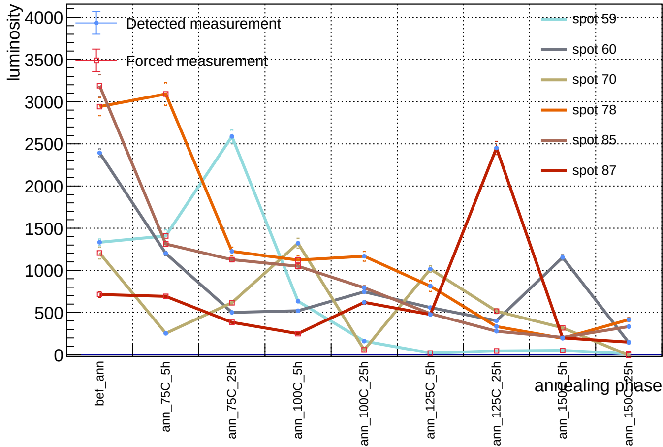
Sensor B1, T = 20 C, v_{\text{over}} = 5 \text{ V} - luminosity vs phase - order 10^3
