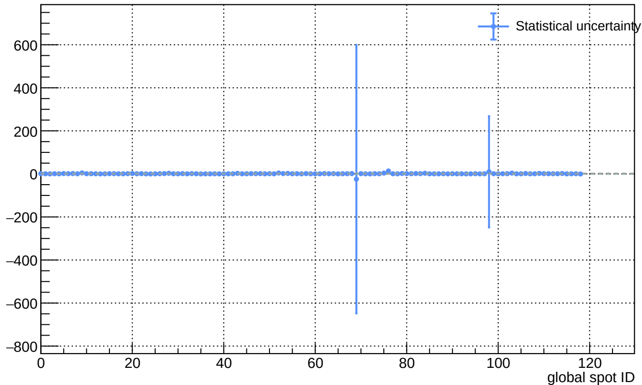
Sensor B1, T = 20 C - L(\text{ann\_100C\_5h}) / L(\text{before\_annealing})
