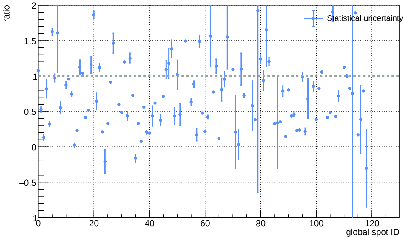
Sensor B1, T = 20\text{ C} - L(\text{ann\_100C\_5h}) / L(\text{before\_annealing})
