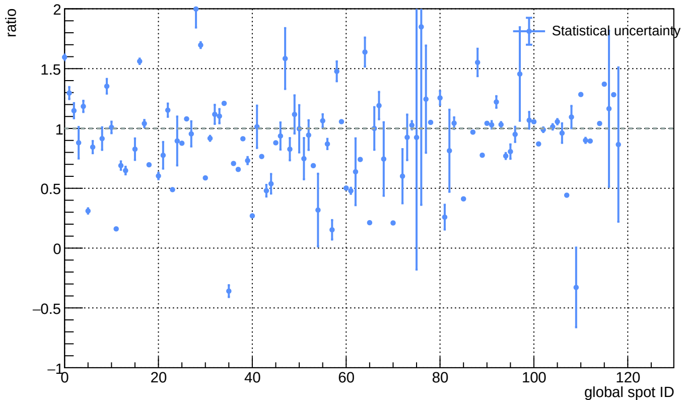
Sensor B1, T = 20 C - L(\text{ann\_75C\_5h}) / L(\text{before\_annealing})
