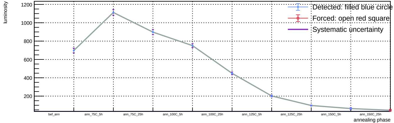
Sensor B1, T = 20\text{ C} , v_{\text{over}} = 5\text{ V} - Spot 0: luminosity vs phase
