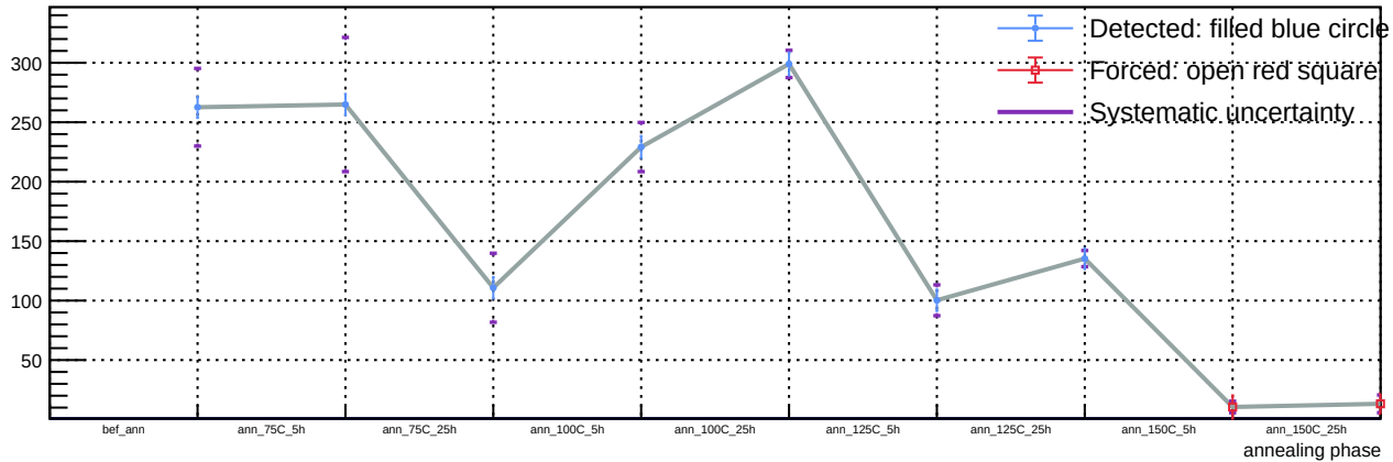
Sensor B1, T = 20\text{ C} , v_{\text{over}} = 5\text{ V} - Spot 10: luminosity vs phase
