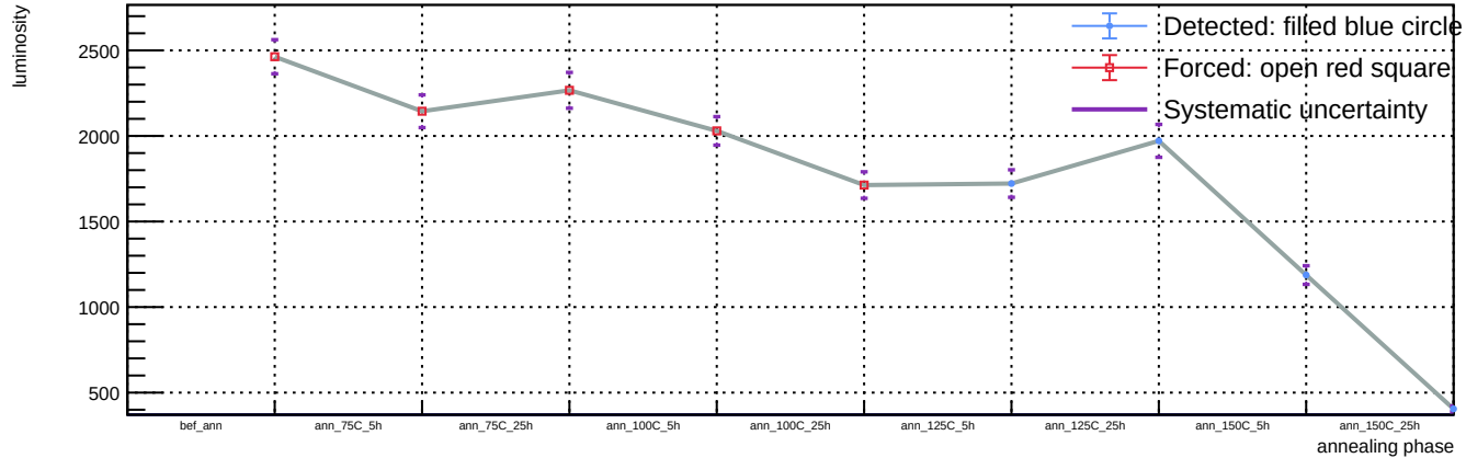
Sensor B1, T = 20 C, v_{over} = 5 V - Spot 101: luminosity vs phase
