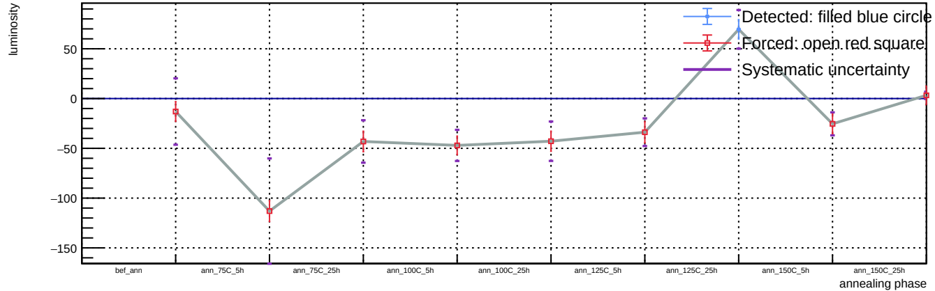
Sensor B1, T = 20\text{ C} , v_{\text{over}} = 5\text{ V} - Spot 103: luminosity vs phase
