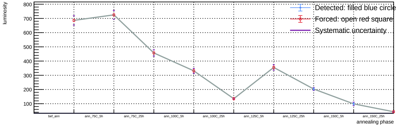
Sensor B1, T = 20\text{ C} , v_{\text{over}} = 5\text{ V} - Spot 105: luminosity vs phase
