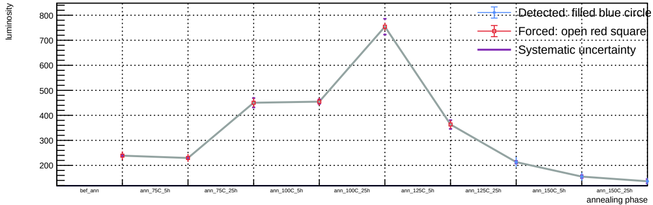
Sensor B1, T = 20 C, v_{\text{over}} = 5 V - Spot 106: luminosity vs phase
