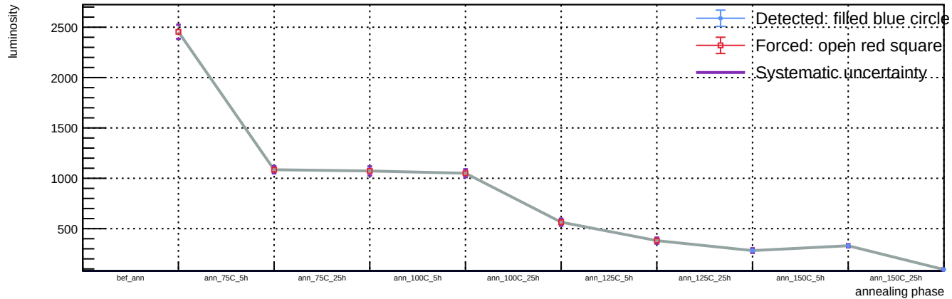
Sensor B1, T = 20\text{ C} , v_{\text{over}} = 5\text{ V} - Spot 107: luminosity vs phase
