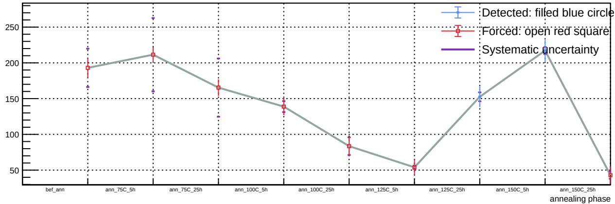
Sensor B1, T = 20\text{ C} , v_{\text{over}} = 5\text{ V} - Spot 108: luminosity vs phase
