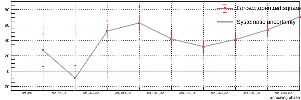
Sensor B1, T = 20\text{ C} , v_{\text{over}} = 5\text{ V} - Spot 109: luminosity vs phase
