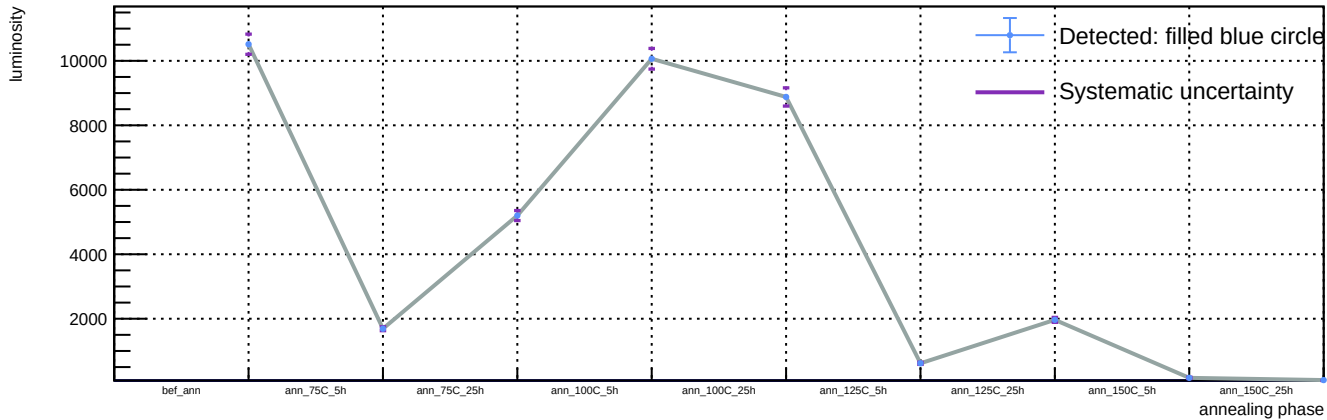
Sensor B1, T = 20\text{ C} , v_{\text{over}} = 5\text{ V} - Spot 11: luminosity vs phase
