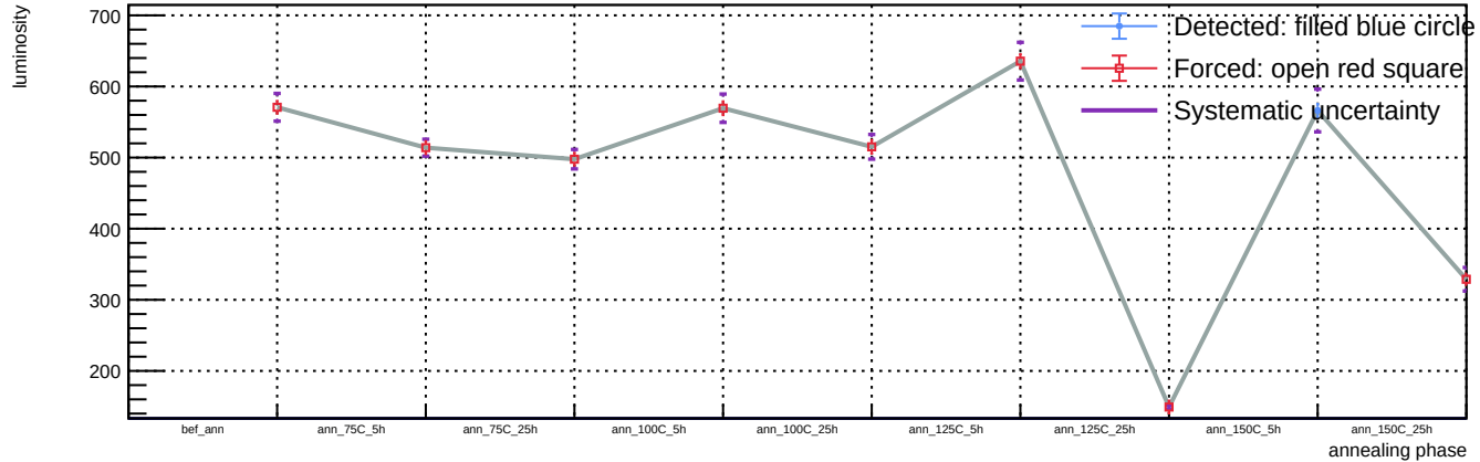
Sensor B1, T = 20\text{ C} , v_{\text{over}} = 5\text{ V} - Spot 111: luminosity vs phase
