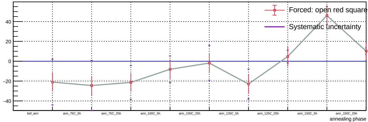
Sensor B1, T = 20\text{ C} , v_{\text{over}} = 5\text{ V} - Spot 116: luminosity vs phase
