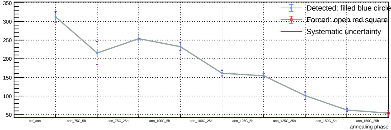
Sensor B1, T = 20\text{ C} , v_{\text{over}} = 5\text{ V} - Spot 12: luminosity vs phase
