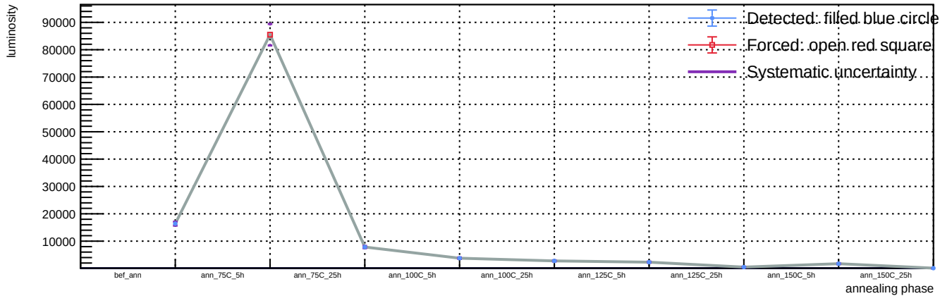
Sensor B1, T = 20\text{ C} , v_{\text{over}} = 5\text{ V} - Spot 14: luminosity vs phase
