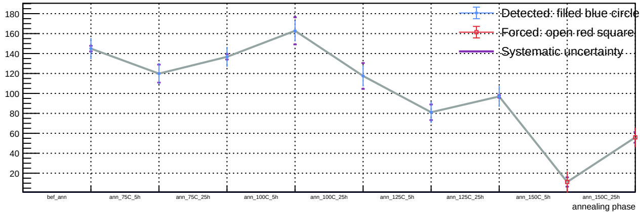
Sensor B1, T = 20\text{ C} , v_{\text{over}} = 5\text{ V} - Spot 15: luminosity vs phase
