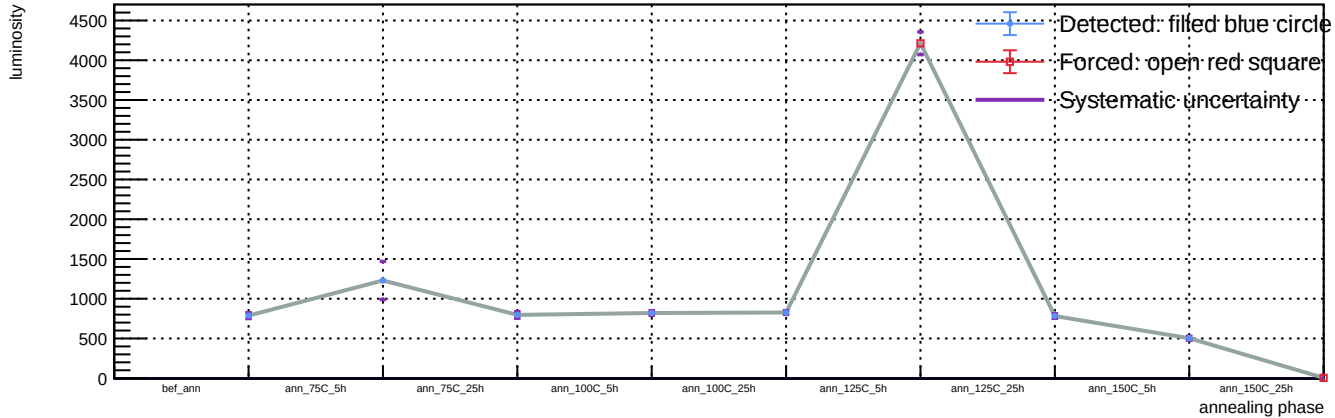
Sensor B1, T = 20\text{ C} , v_{\text{over}} = 5\text{ V} - Spot 16: luminosity vs phase
