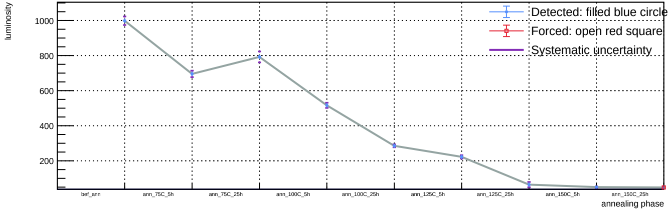
Sensor B1, T = 20\text{ C} , v_{\text{over}} = 5\text{ V} - Spot 18: luminosity vs phase
