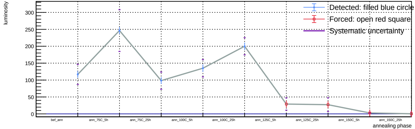
Sensor B1, T = 20\text{ C} , v_{\text{over}} = 5\text{ V} - Spot 19: luminosity vs phase
