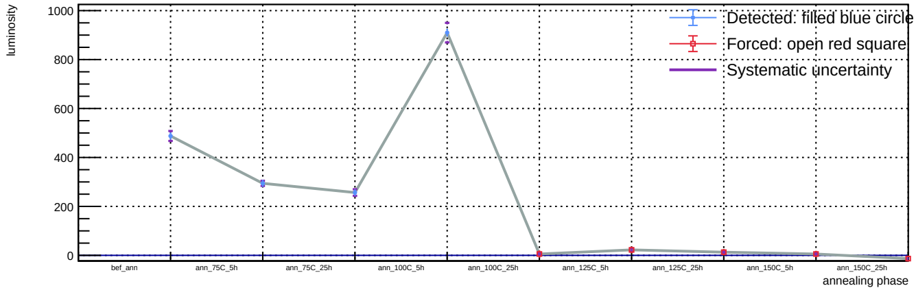
Sensor B1, T = 20\text{ C} , v_{\text{over}} = 5\text{ V} - Spot 20: luminosity vs phase
