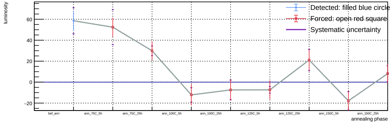
Sensor B1, T = 20\text{ C} , v_{\text{over}} = 5\text{ V} - Spot 24: luminosity vs phase
