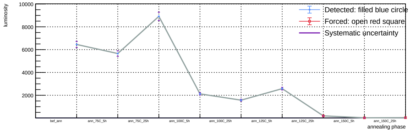
Sensor B1, T = 20\text{ C} , v_{\text{over}} = 5\text{ V} - Spot 25: luminosity vs phase
