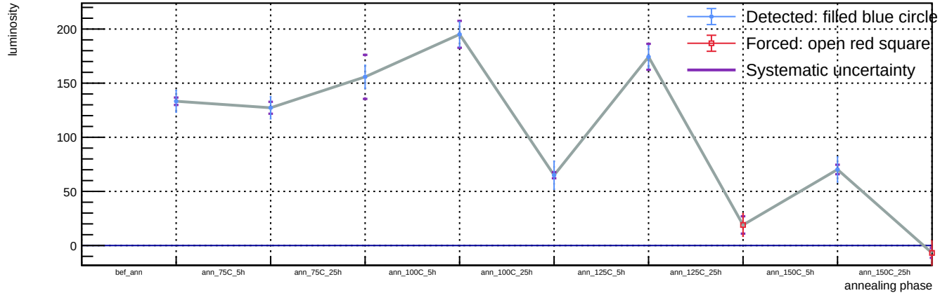
Sensor B1, T = 20\text{ C} , v_{\text{over}} = 5\text{ V} - Spot 27: luminosity vs phase
