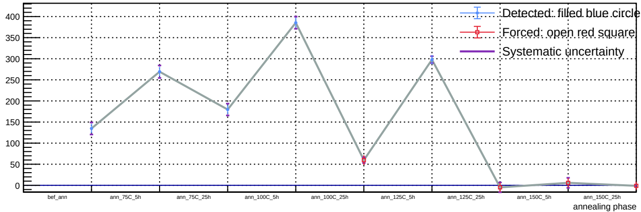
Sensor B1, T = 20\text{ C} , v_{\text{over}} = 5\text{ V} - Spot 28: luminosity vs phase
