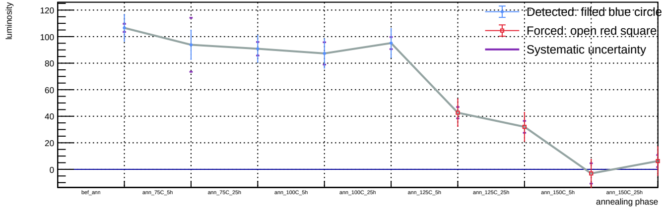
Sensor B1, T = 20\text{ C} , v_{\text{over}} = 5\text{ V} - Spot 3: luminosity vs phase
