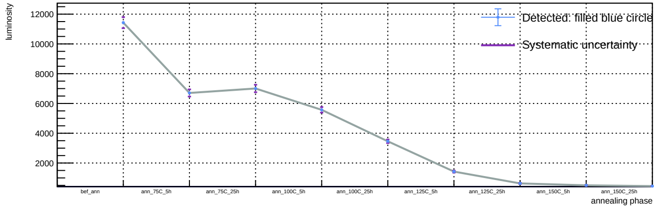
Sensor B1, T = 20\text{ C} , v_{\text{over}} = 5\text{ V} - Spot 30: luminosity vs phase
