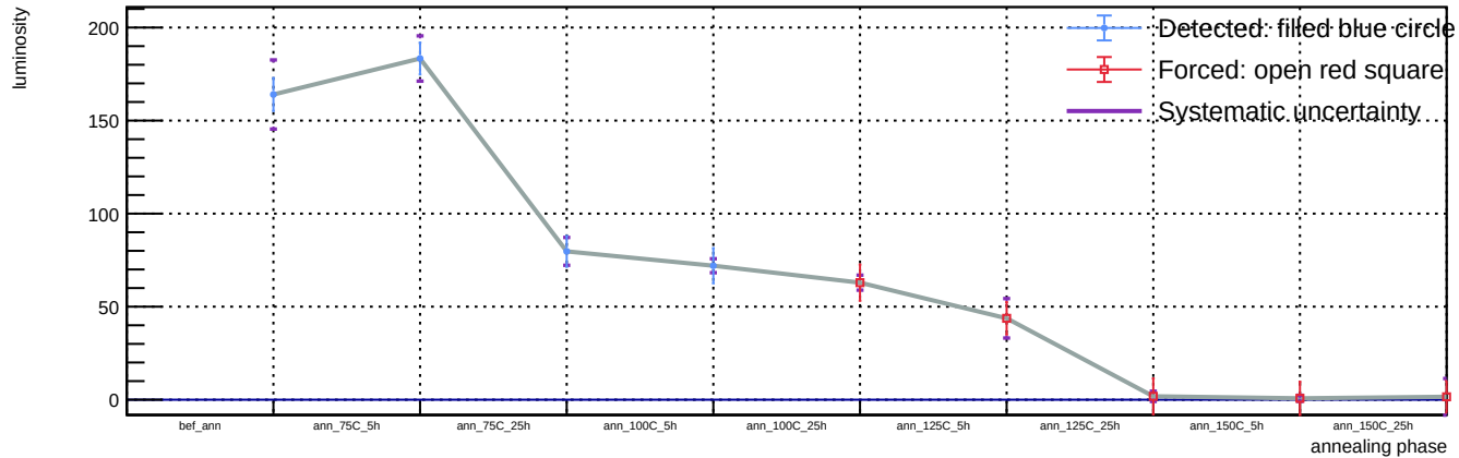
Sensor B1, T = 20\text{ C} , v_{\text{over}} = 5\text{ V} - Spot 32: luminosity vs phase
