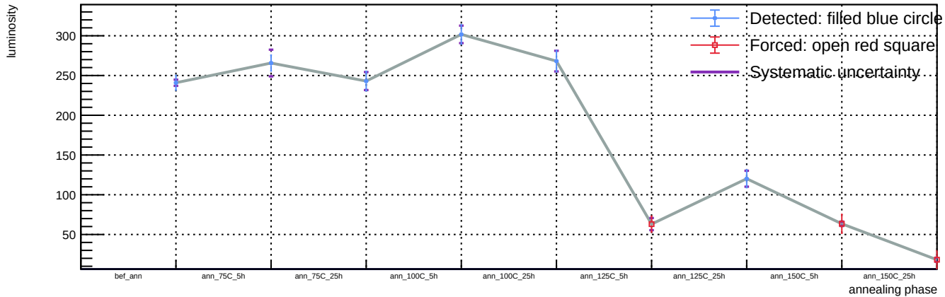
Sensor B1, T = 20\text{ C} , v_{\text{over}} = 5\text{ V} - Spot 33: luminosity vs phase
