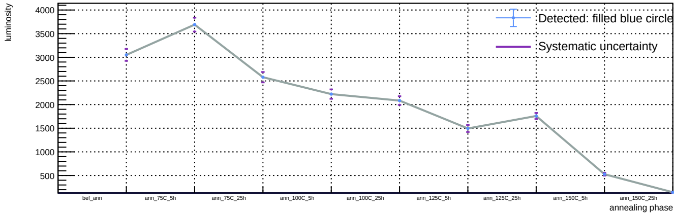
Sensor B1, T = 20\text{ C} , v_{\text{over}} = 5\text{ V} - Spot 34: luminosity vs phase
